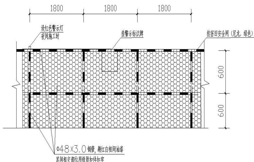
钢管护栏大样
